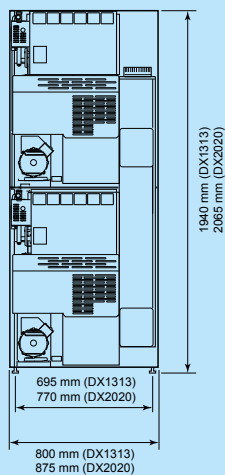
Side DX 13/13 20/20
